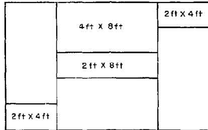
1.a TYPICAL LAYOUT FOR ROOF. 4 UNCLUT SHEETS, ONE SHEET CUT TO PRODUCE ONE 2 ft X 8 ft AND TWO 2 ft X 4 ft PIECES. (TOTAL REQUIRED = 10 SHEETS)
